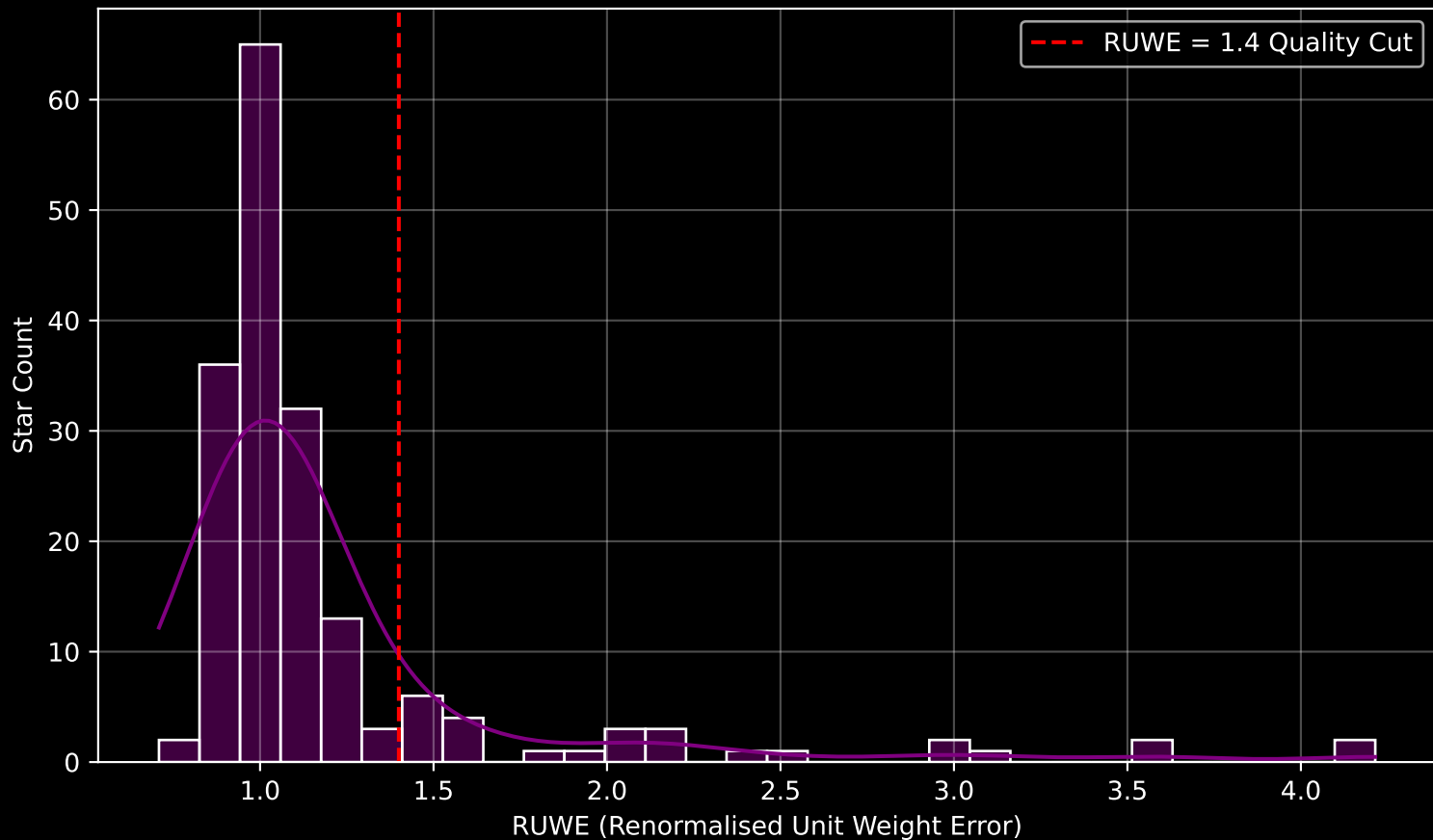
GAPOGEE DR17 Field [189+49_MGA] RUWE Distribution (n= 178)
