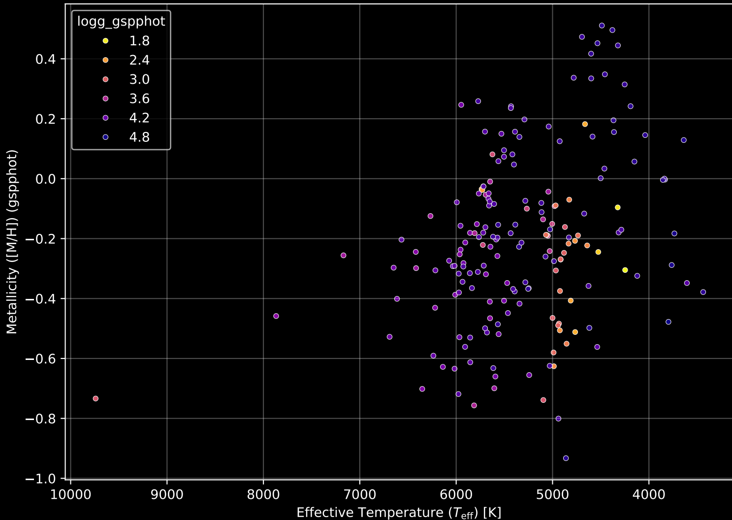
APOGEE DR17 Field: [189+49_MGA] Stellar Population Parameters (n= 185)
