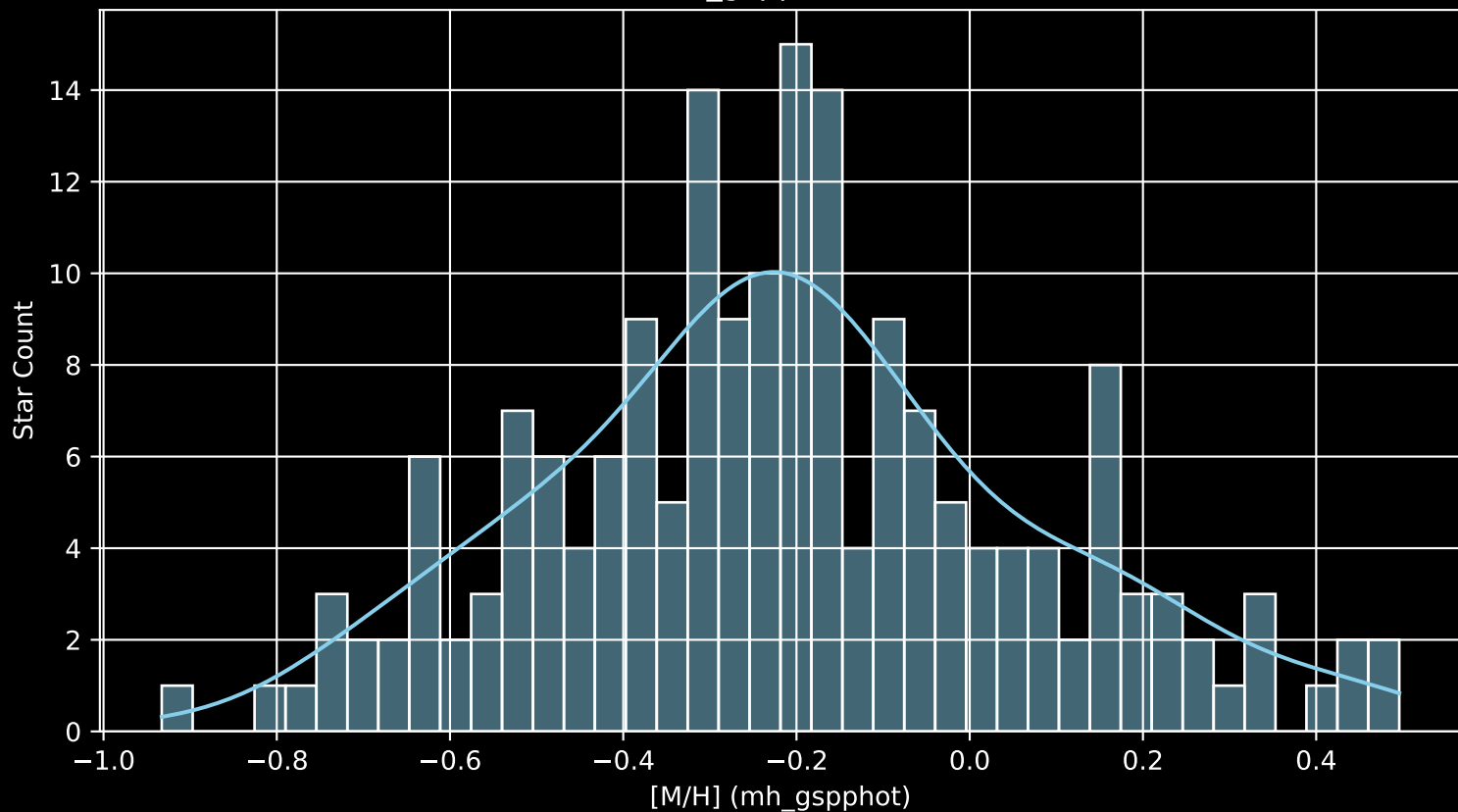
APOGEE DR17 Field: [189+49_MGA [M/H] (mh_gspphot) (n= 184)
