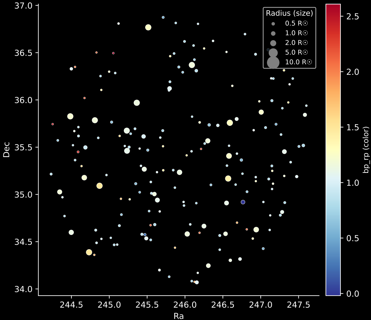
APOGEE DR17 Field: [189+49_MGA] Stars: 185
