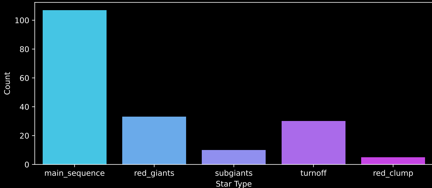
APOGEE DR17 Field: [189+49_MGA] Count plot of Star Type
