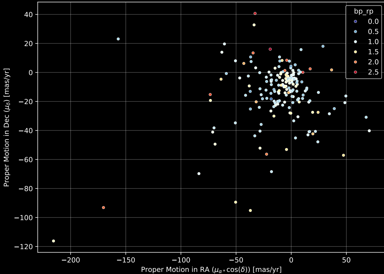
APOGEE DR17 Field: [189+49_MGA] Proper Motion Diagram (n= 185)
