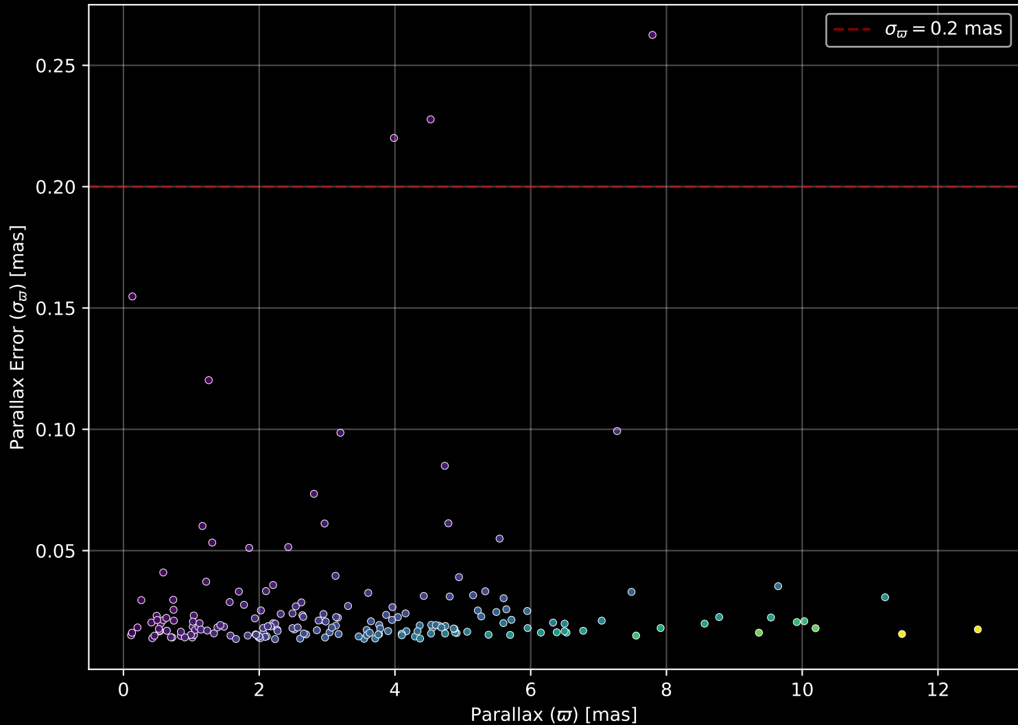
APOGEE DR17 Field: [189+49_MGA] Parallax Quality (n= 185)
